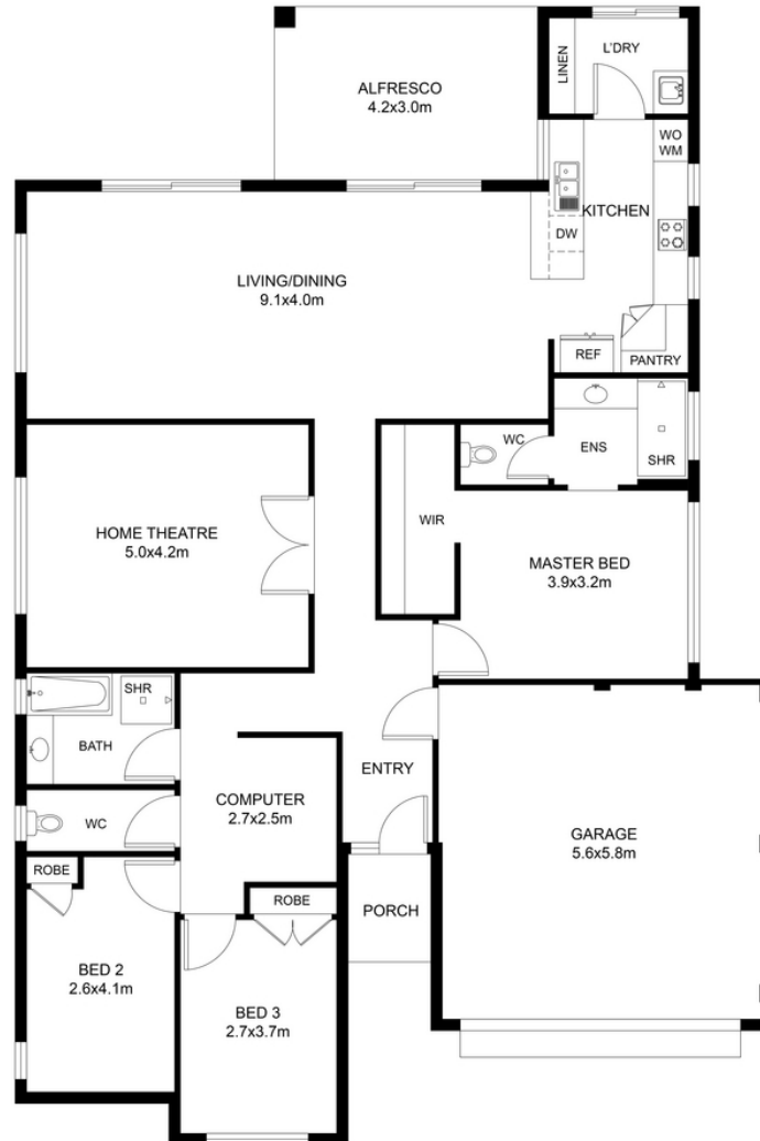
FLOOR PLAN
